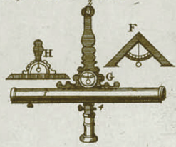
Fig. 6 Plumb Level
